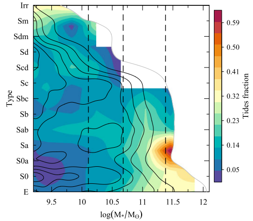
Figure 20. Bivariate distributions in the T -TYPE- M_* diagram (similar to Fig. 19) coloured by the tides fractions.
