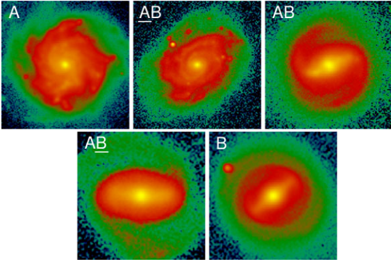
Figure 3. Bar family classification examples following the CVRHS system (R. J. Buta et al. 2015). From left to right: (A) no-barred galaxy, ( AB ) weak bar showing a roundish structure, ( AB ) bar in the inner region of the galaxy, ( AB ) clear conspicuous bar, and (B) bar with high contrast with respect to other structures. Note that AB , AB , and B families are strong bars. See more details in Section 2.1.2.
