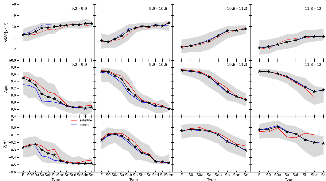
Figure 15. Stars and error region are the same as in Fig. 14. Red lines show the median of the satellite galaxies for every property as a function of morphology, and the blue line the median of the central galaxies sample.
