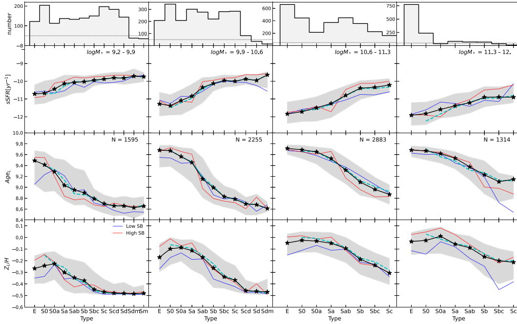
Figure 14. Upper panels: the morphological types histogram in four stellar mass bins. To avoid biased statistics, only bins with more than 10 galaxies are considered in this figure. As reference, dotted line shows the level at 50 galaxies. Middle-upper panels: sSFR as a function of morphological type. Stars represent the median in each bin, and the grey shadow region is the error associated with the 0.16 and 0.84 percentiles. To see a correlation with the mean SB ( \mu = m + 2.5 \times \log(A) ), we consider the median of the sample below the 0.16 percentile of SB (blue lines) and the above the 0.84 percentile of SB (red lines). Dashed cyan lines show the median corresponding to the barred galaxies sample. Lower middle and lower panels: stellar population light-weighted age and stellar population light-weighted metallicity in terms of the morphological types. Symbols and lines are similar to upper panels.
