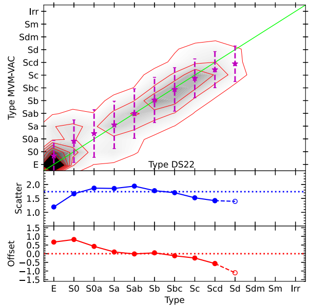
Figure 17. Upper panel: DS22 classification versus the visual classification in this work in 2D density histograms normalized to the total number of the sample. Isocontours are presented in lineal scale and the most external is formed with bins containing at least 0.5 per cent of the sample (50 galaxies). The one-to-one line is presented in green and the average with the standard deviation (magenta) for each morphology in DS22. Lower panel shows our relative offset of the average with respect to the one-to-one line (red), and scatter with respect to the average (standard deviation; blue) for a given morphological bin in DS22. Dotted lines (blue) are the median estimated from all values of scatter for types \leq Scd, and the zero-point reference for the offset (red). Later types than Scd (dashed and open circles) are omitted due to the low number of galaxies in these bins.
