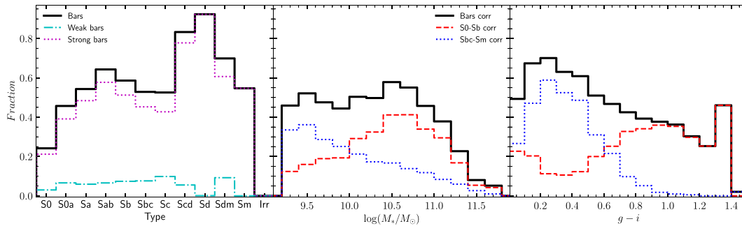
Figure 7. Fractions per bin (volume-corrected) of barred galaxies (solid-black lines) as functions of morphology, stellar mass, and g-i colour. The first panel show the fraction distribution separated in Bar families: strong bars (AB, AB, and B) in dotted-magenta and weak bars (AB) in cyan-dashed line. The last panels present the fraction distributions divided into early (S0–Sb; red-dashed line) and late (Sbc–Sm; blue-dotted line) type discs. Note: fraction distribution are defined as the number of barred galaxies in each bin divided by the total number of galaxies in that bin. Only galaxies with inclinations < 70^\circ are considered. Galaxy colours are corrected as described in Section 4.2.
