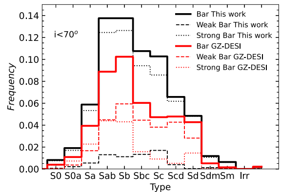
Figure 18. Barred galaxies distribution as a function of morphology, for bars detected in this work (solid black) and those identified in the GZ-DESI catalogue (solid red), in the common disc sample. We also separate the weak (dashed line) and strong (dotted line) bars according to the GZ-DESI (red) and this work (black) bar identification. These distribution are normalized to the 3298 discs in common with the GZ-DESI catalogue.
