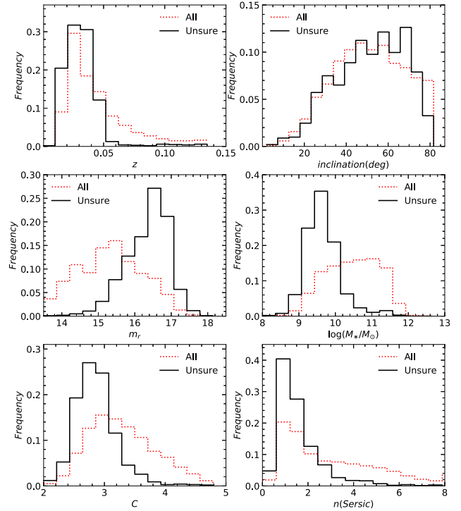
Figure D1. Frequency distribution of galaxies difficult to classify (‘unsure’; solid line) as a function of redshift, inclination, r -band apparent magnitude, stellar mass, concentration ( C ), and Sérsic index. As reference, red dotted lines show the distributions for the whole MaNGA DR17 sample. All these distributions are normalized to the total number in every sample.
