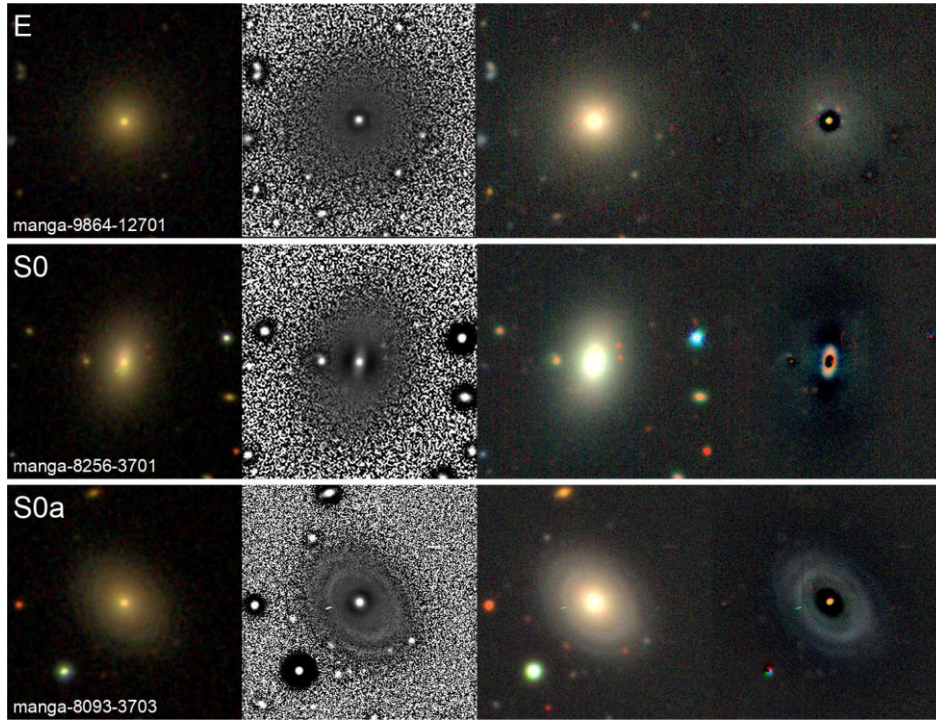
Figure 1. Poster-child of our classification scheme for early E, S0, and S0a types. For every mosaic, columns from left to right show the gri SDSS image, the filtered-enhanced r -band DESI image, the grz DESI image, and the residual DESI image after a best 2D SB model subtraction.
