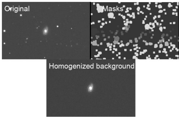
Figure 4. Background replacement and homogenization of images (see Section 2.2) previous to CAS estimates. Panels: original image, computed masks, background replacement, and homogenization.
