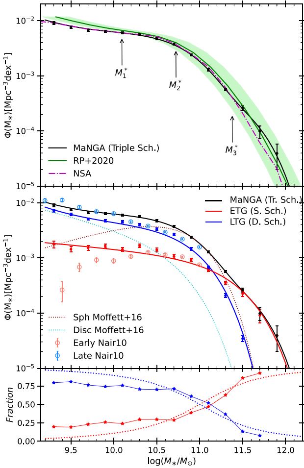
Figure 11. Upper panel: GSMF for the MaNGA sample (black dots) with its best-fitting (black line) considering a triple Schechter function. Errors are estimated through a bootstrap approach in a set of 8000 randomly selected samples, with the size of the original sample. The arrows indicate the three corresponding characteristic masses. As comparison, the the NSA catalogue GSMF (magenta dot-dashed line) and SDSS DR7 + low- z SDSS GSMF fit according to RP20 (green line) are plotted. The shadow region represents the uncertainty due to the systematic uncertainties in the M_* estimate. Middle panel: the MaNGA GSMF divided into ETGs (red circles), and LTGs (blue circles), fitted by a single and double Schechter function, respectively (blue and solid lines). As comparison, the GAMA GSMFs for spheroids and discs (dotted lines; A. J. Moffett et al. 2016) and the P. B. Nair & R. G. Abraham (2010) GSMF for ETG and LTG (open circles) are reproduced. Lower panel: the early and late GSMF divided by the total MaNGA GSMF (red and blue asterisks and solid lines, respectively), and as comparison the fractions reported by RP20 (dotted lines). Note that estimations and comparisons are corrected to the cosmology used in this paper.
