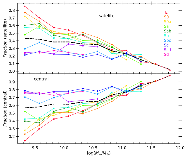
Figure 16. Top panel: fraction of satellite galaxies as a function of stellar mass (black dashed line) and for each morphological type (colour solid lines). Bottom panel: same as in the top panel, but for the central galaxies.
