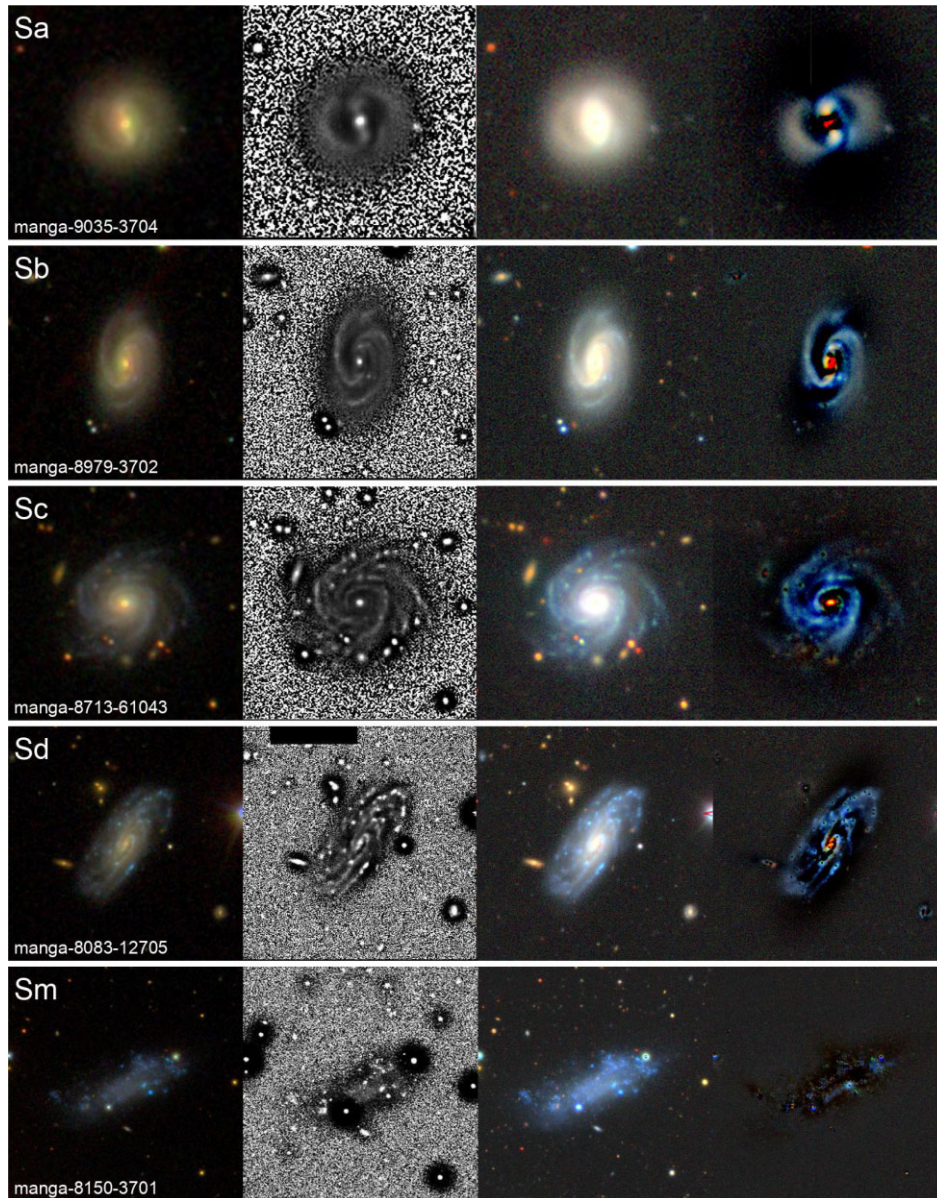
Figure 2. Poster-child of our late-type classification scheme from Sa to Sm. Mosaics are similar to those in Fig. 1.
