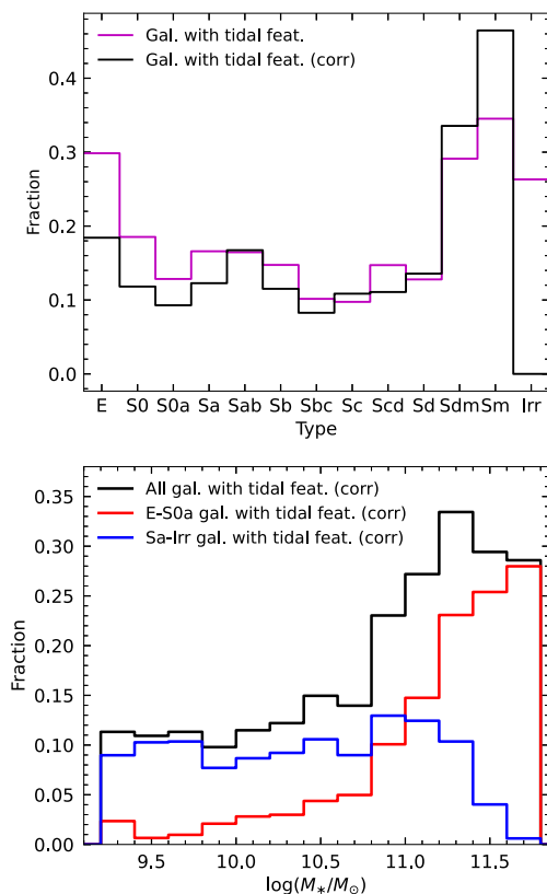
Figure 8. Distribution of the fraction of galaxies with tidal features per bin of morphology (upper panel) and stellar mass (lower panel), for the original (solid-magenta line) and volume-corrected (solid-black line) samples. Tidal debris are divided into early (red) and late (blue) types in the lower panel. Note that these fractions mean the number of galaxies with tidal features in each bin divided by the total number of galaxies in the same bin.
