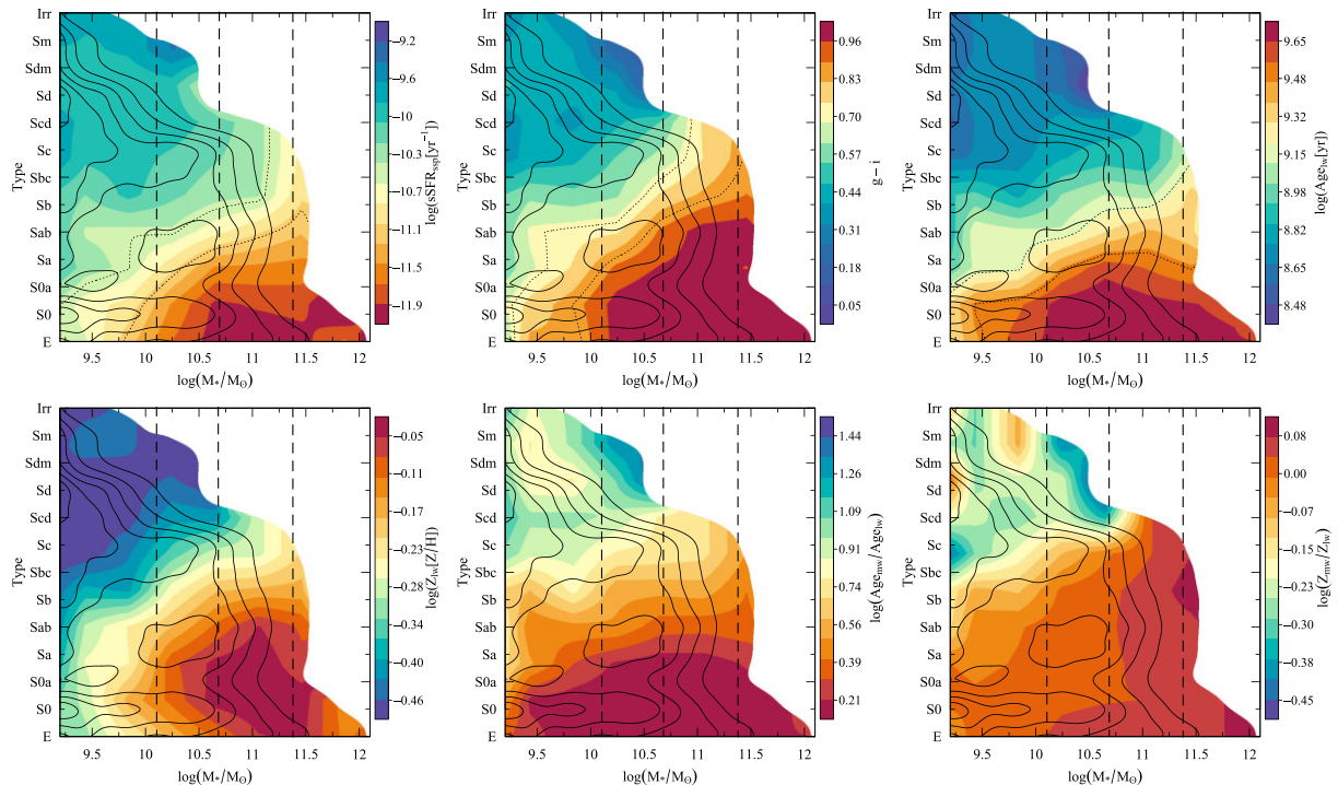
Figure 13. Bivariate distributions in the T -TYPE- M_* diagram (isodensity contours and dashed lines are the same as right-hand panel in Fig. 6) but coloured by the sSFR (upper left panel), the dust-corrected g-i colour (upper central panel), the luminosity-weighted age (upper right panel), the luminosity-weighted metallicity (lower left panel), the ratios of the mass- to luminosity-weighted mean ages (lower central panel), and metallicities (lower right panel) as indicated in the colour bars, respectively. The dotted lines indicate the transition zones in \log(\text{sSFR}/\text{yr}) [-10.5, -11.1] , g-i colour [0.70-0.85] mag, and \log(\text{Age}_{\text{lw}}/\text{yr}) [9.18-9.48] .
