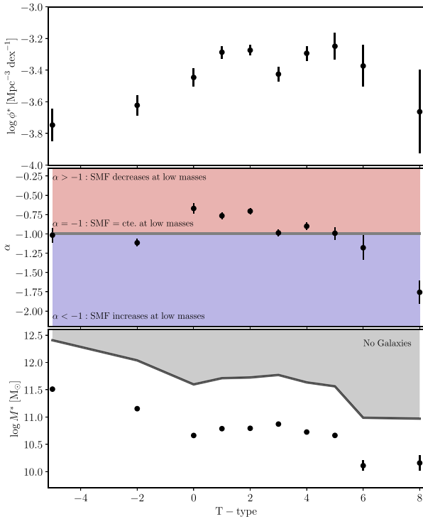
Figure 22. Upper panel: the GSMF fitted normalization from a single Schechter function fit, \phi^* . Middle panel: the GSMF fitted slope ( \alpha ). The grey solid line represents the case when \alpha = -1 , for values \alpha > -1 , the number density of galaxies decreases as mass decreases, whereas for \alpha < -1 , the number density of galaxies increases. Note that Scd–Irr morphological types, which dominate the low-mass end of the GSMF, become more prevalent at lower masses. Lower panel: The GSMF fitted characteristic stellar mass ( M^* ). The solid dark grey line represents the stellar mass at which the GSMF decreases by three orders of magnitude compared to the number density of M^* galaxies. The probability to observe such galaxies is less than \sim 2 \times 10^5 when accounting galaxies with stellar masses M_* \geq 10^9 M_\odot . Equivalently, to observe at least one of such galaxies volumes of (\sim 0.4 \text{ Gpc})^3 are needed. These values are reported in Table 6.
