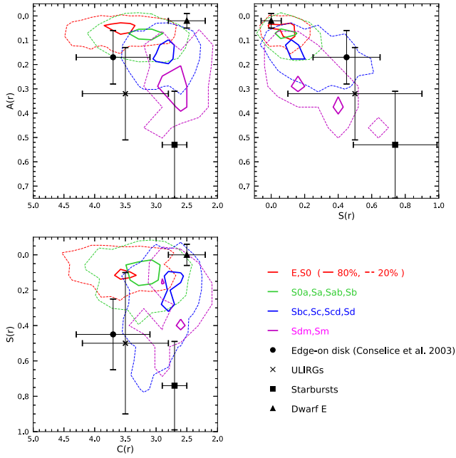
Figure 9. CAS parameters in two levels contour plots (solid lines = 0.8 and dotted lines = 0.2), for early (red), intermediate (green), late (blue), and very late (magenta) types. As comparison (in black symbols), we mark the position of edge-on, ULIRGs, starbursts and dwarfs ellipticals according to C. J. Conselice (2003). Note that these plots only consider galaxies with low inclinations ( < 70^\circ ) and within the following interval values: 0 < A < 0.5 , 2 < C < 5 , and -0.2 < S < 0.8 , according to different authors (e.g. M. M. Pawlik et al. 2016).
