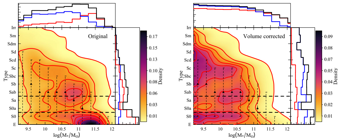
Figure 6. Bivariate distribution of the MaNGA galaxies with i \leq 70^\circ in the morphological type versus M_* diagram, not taking (left panels) and taking (right panels) into account volume completeness corrections. The bivariate densities are shown with the isocontours and colours in linear scale representing a fraction from the total sample, with the last isocontour equivalent to 0.0005 of the normalized number density. Filled triangles and bars show the median and quartiles in morphology given a stellar mass bin. Horizontal dashed lines show the transition zone of the bimodal distribution. The top and right histograms in each panel show the 1D distributions of stellar mass and morphology. These are divided by ETG (red) and LTG (blue) and by massive ( \log(M_*/M_\odot) \geq 10.5 ; red line), and low massive ( 9.2 \leq \log(M_*/M_\odot) < 10.5 ; blue line) galaxies. The raster figures are constructed from a regular grid of 10 \times 10 bin in all the diagram intervals. At the centre of each pixel, we obtained the weighted median of the number density galaxy population, considering the entire sample, by associating weights to each galaxy according to a bivariate normal distribution. The kernel widths of the bivariate distribution in the x - and y -directions are obtained automatically following B. W. Silverman (1986) rule. Note the volume corrections are additionally considered. For more details, see Appendix B.
