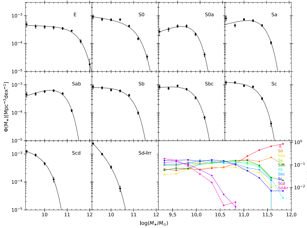
Figure 12. The GSMF of each morphological type and their fits using a simple Schechter function (solid black line); for the best-fitting parameters, see Table 6. Bottom-right panel shows the fraction of each type as a function of M_* , \phi_i/\phi , where i = \text{T-TYPE} .
