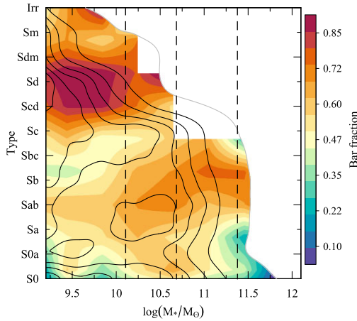
Figure 19. Bivariate distributions in the T -TYPE- M_* diagram (isodensity contours and dashed lines are the same as right-hand panel in Fig. 6) coloured by the bar fractions.
