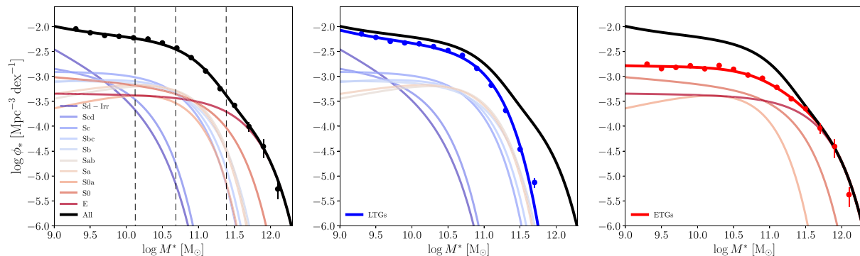
Figure 21. Contribution of each morphological type to the total GSMF (left panel), of types Sa–Irr to the LTG GSMF (medium panel), and of types E–S0a to the ETG GSMF (right panel). The light coloured lines represent the best single Schechter fits for each morphological type as in Fig. 12, black line is the sum of all of them, while blue and red lines are the sum of the fits to only the Sa–Irr and E–S0 GSMFs, respectively. The black, blue, and red filled circles show the observed total, LTG, and ETG GSMFs. The former is best described by a triple Schechter function (see Section 4 and Table 5) with characteristic masses of M_1^* \approx 1.2 \times 10^{10} M_\odot , M_2^* \approx 5.3 \times 10^{10} M_\odot , and M_3^* \approx 2.4 \times 10^{11} M_\odot (dashed lines). The first mass is dominated by galaxies with morphologies later than Scd, the intermediate mass is dominated by S0a–Sc types, and the last mass is primarily dominated by E galaxies. The GSMF for LTGs follows a double Schechter function, while ETGs exhibit a more complex shape but can be roughly approximated by a Schechter function with a large characteristic mass, \approx 2.4 \times 10^{11} M_\odot . At lower masses, the total and LTG GSMFs are dominated by the steep slope of the Sd–Irr morphological types.
