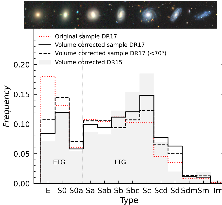
Figure 5. Morphology histogram showing the results of the classification carried out in this work. Every distribution represents the complete MaNGA sample (dotted-red line), the volume-corrected sample (solid-black line), the corresponding volume-corrected sample excluding galaxies with inclinations > 70^\circ (dashed-black line), and the previous distribution presented in Paper I for the DR15 MaNGA sample (shadow grey area). Note that (i) these distributions are normalized to the total number of galaxies in each sample, and (ii) the volume-corrected distributions, only galaxies with \log(M_*/M_\odot) \geq 9.2 are considered. The vertical dotted line illustrates the separation between ETG and LTG adopted in this work.
